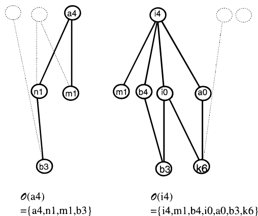
Figure 3. Examples of principal order ideals, each generated by exactly one element of P' . To facilitate the identification some other objects and edges are indicated.
