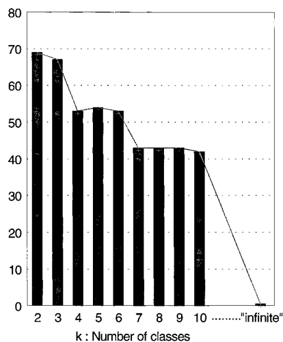
Figure 5. D(\mathcal{A}^o, \mathcal{A}^{ec}) is shown in dependence of k . The same k for each of the three properties. The fine line helps to identify the only one local minimum and a series of constant values.
